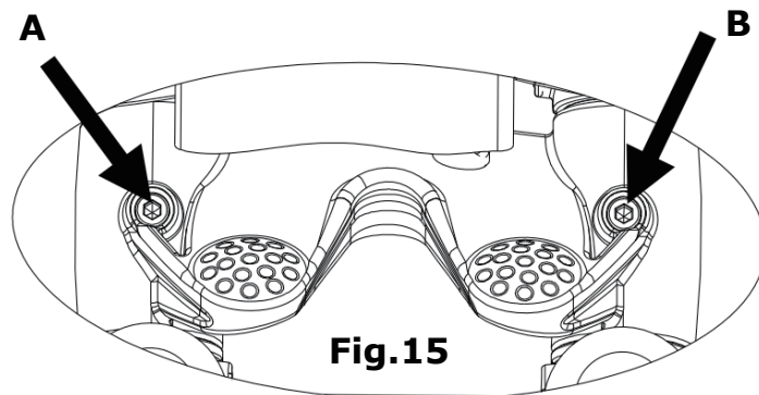
Alignment adjusting screws A/B
